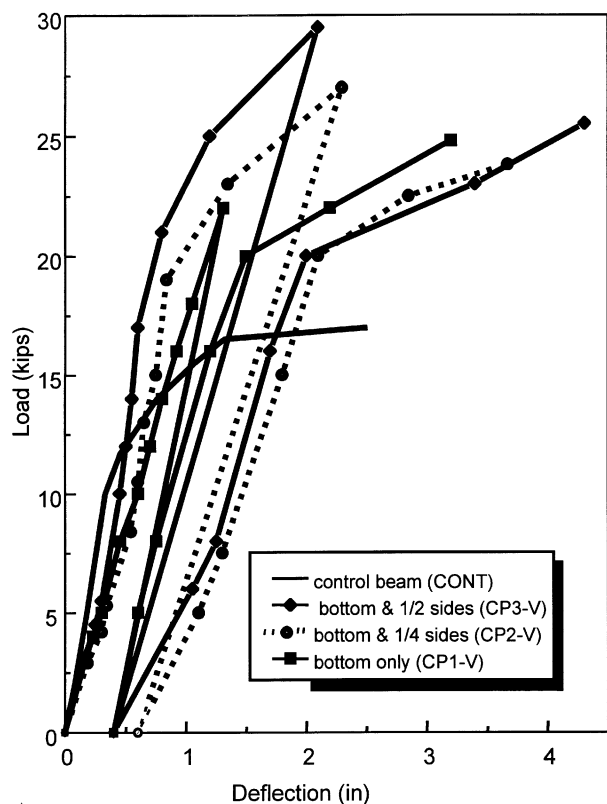
Fig. 6—Response of Group 5 strengthened beams.
