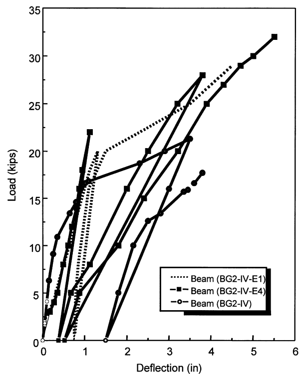
Fig. 5—Response of Group 4 strengthened beams.
