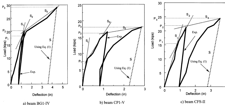
Fig. 9—Comparison between theoretical and experimental unloading slopes: (a) Beam BG1-IV; (b) Beam CP1-V; and (c) Beam CFS-II.
