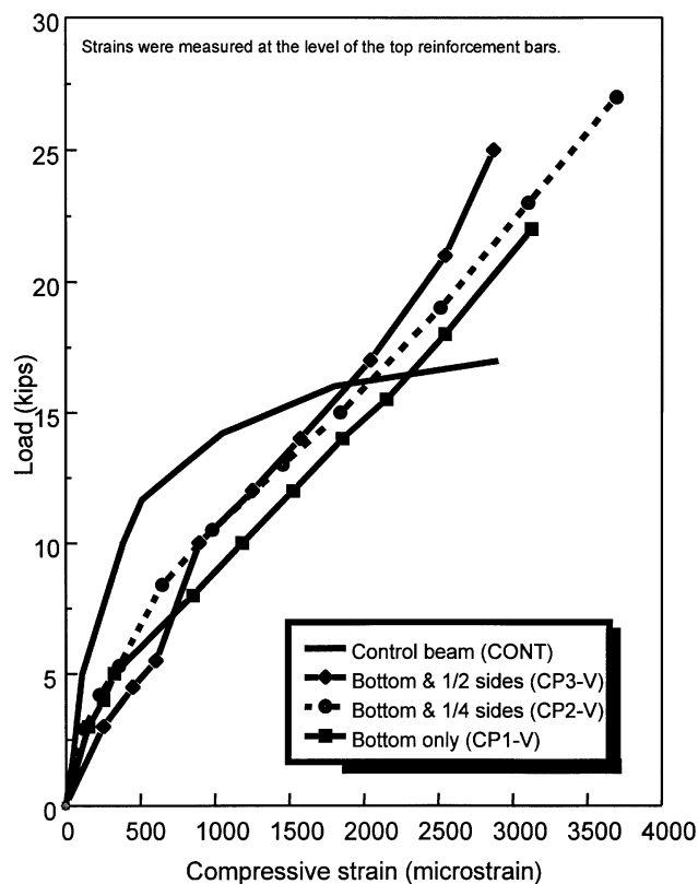
Fig. 7—Strain response of Group 5 beams during first cycle of
